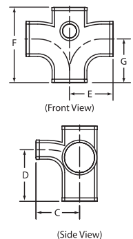
Edge HP Sanitary Cross (New Orleans Code, with 2" 90° Sanitary Inlet Above Center)
