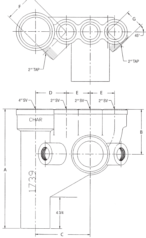
Right Hand Vented Closet Tee with 2" 45° Taps (Designed for use above the floor)
