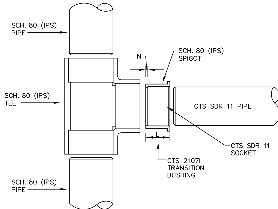
CTS PART NO. 21071 TRANSITION BUSHING
