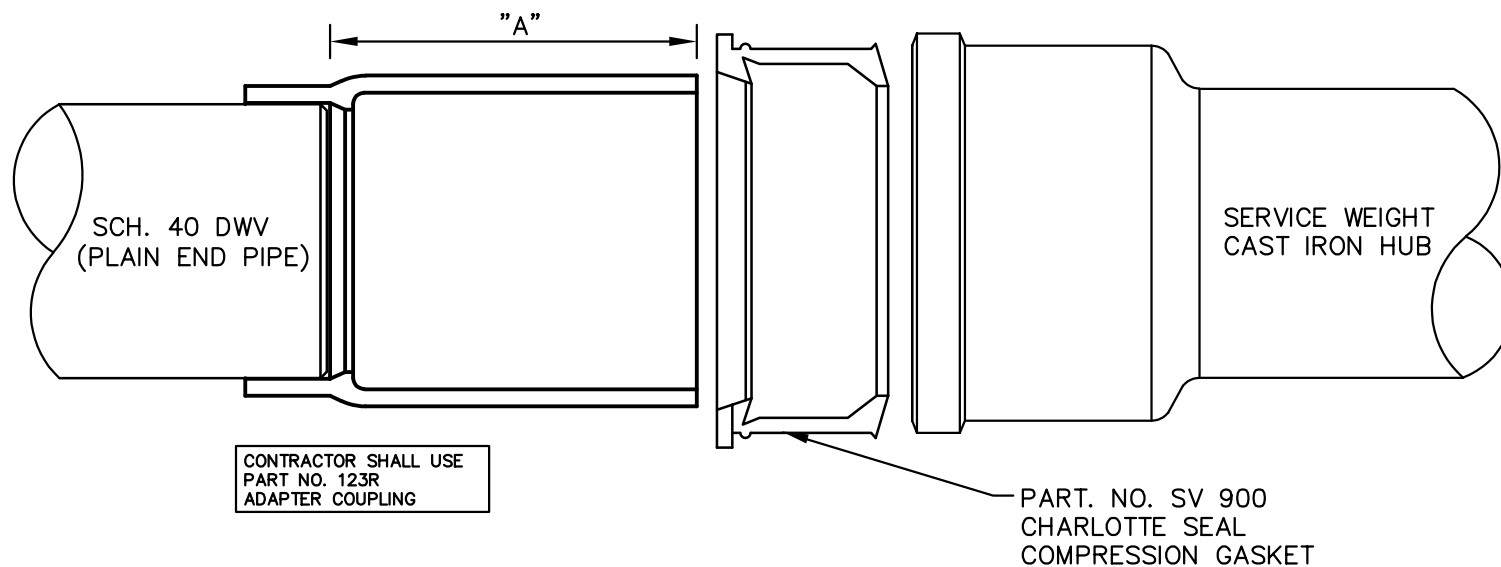
PART NO. 123R REDUCING ADAPTER HUB x SPIGOT (ADAPTS DWV SPIGOT TO CAST IRON HUB)
