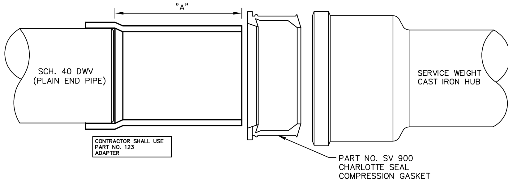
PART NO. 123 ADAPTER HUB x SPIGOT (ADAPTS DWV SPIGOT TO SV CAST IRON HUB)
