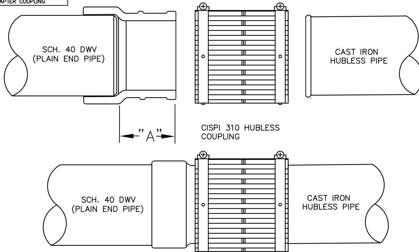
PART NO. 119 ADAPTER COUPLING SPIGOT X HUB (ADAPTS CAST IRON HUBLESS SPIGOT TO DWV SPIGOT)
