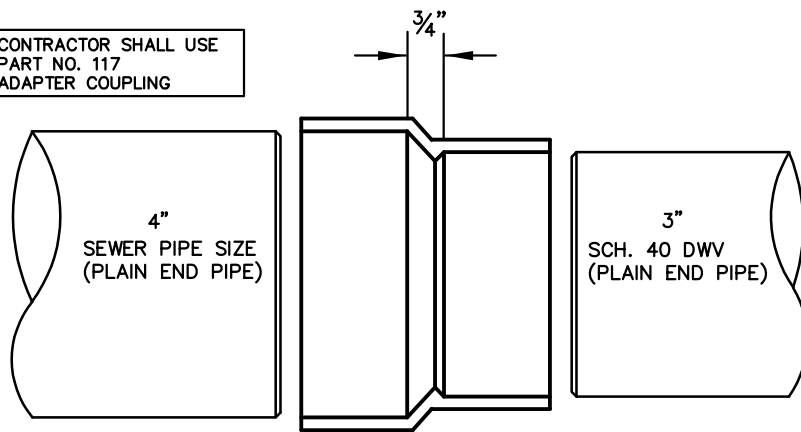
PART NO. 117 4"X3" ADAPTER COUPLING SEWER HUB x DWV HUB (ADAPTS SEWER AND DRAIN SPIGOT TO DWV SPIGOT) AVAILABLE IN PVC AND ABS
