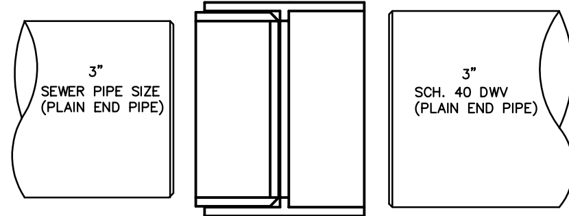
PART NO. 117 3"X3" ADAPTER COUPLING SEWER HUB x DWV HUB (ADAPTS SEWER AND DRAIN SPIGOT TO DWV SPIGOT) ASSEMBLED PART USING PART #118 INTO PART #100 AVAILABLE IN PVC ONLY
