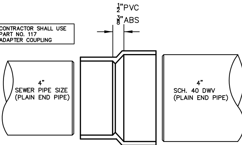
PART NO. 117 4"X4" ADAPTER COUPLING SEWER HUB x DWV HUB (ADAPTS SEWER AND DRAIN SPIGOT TO DWV SPIGOT) AVAILABLE IN PVC AND ABS
