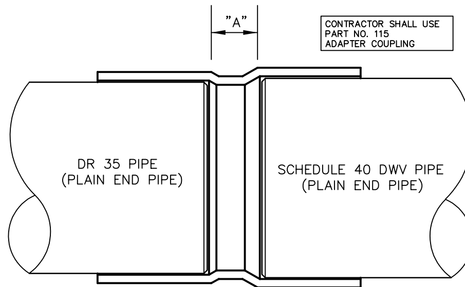
PART NO. 115 ADAPTER COUPLING DR 35 HUB x DWV HUB
